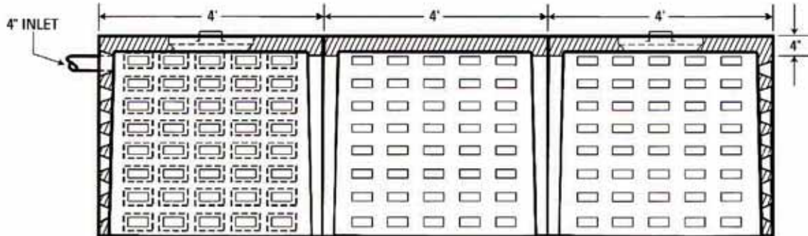
TYPICAL CENTER SECTION 40 - 2"X5" OPENINGS EACH SIDE
